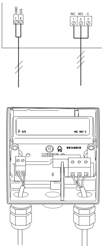
Fig. 2 Cable connection
